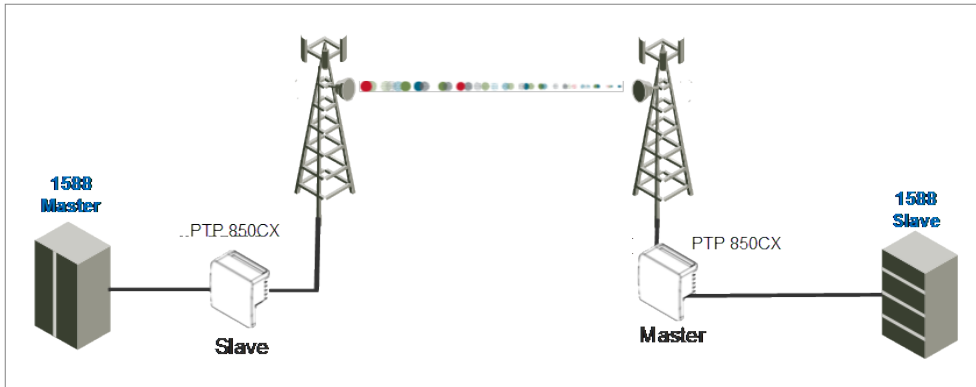
Figure 53: Boundary Clock – General Architecture
