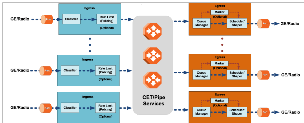
Figure 38: QoS Block Diagram
