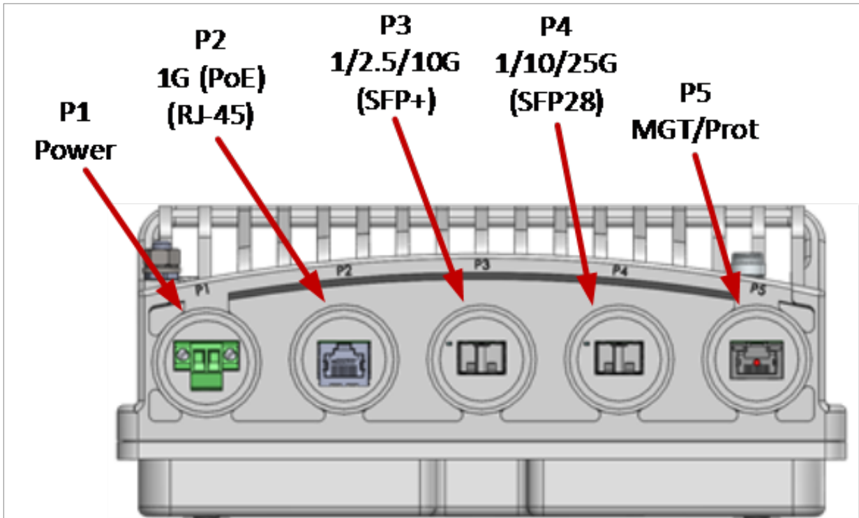
Figure 2: PTP 850CX Interfaces
