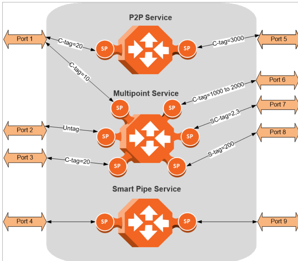
Figure 24: PTP 850CX Services Core
