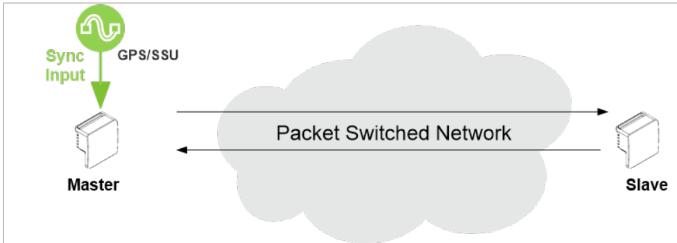
Figure 49: IEEE-1588v2 PTP Optimized Transport – General Architecture
