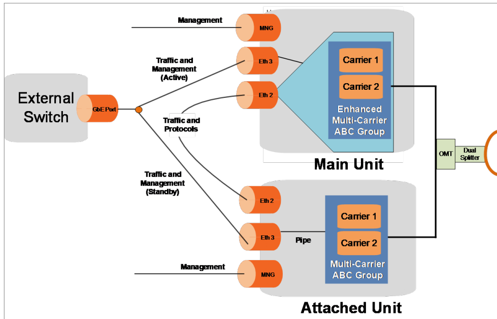
Figure 14: 4+0 PTP 850CX with Layer 1 Link Aggregation and Line Redundancy
