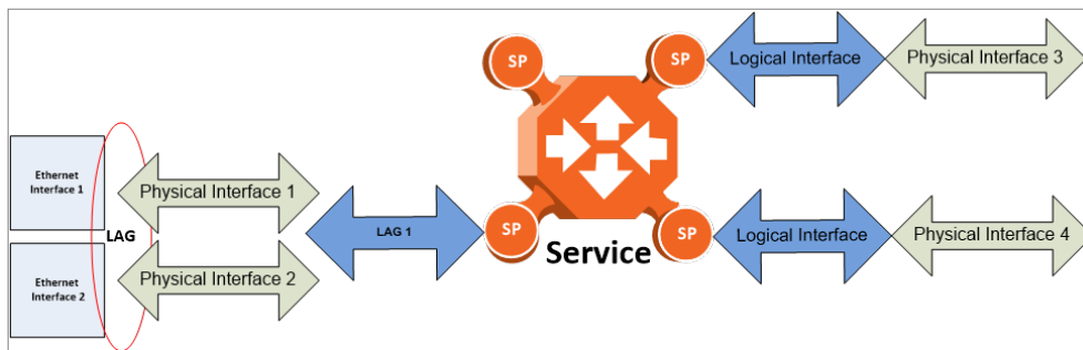
Figure 37: Relationship of Logical Interfaces to the Switching Fabric
