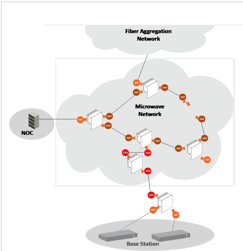
Figure 32: SAP, SNP and Pipe Service Points in a Microwave Network
