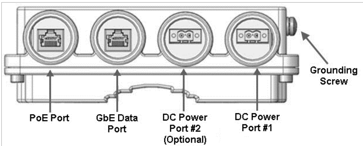
Figure 6: PoE Injector Ports
