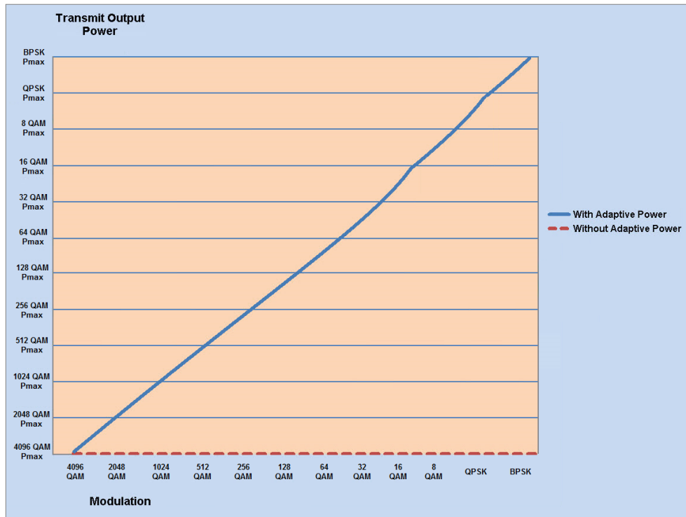
Figure 17: PTP 850CX ACM with Adaptive Power Contrasted to Other ACM Implementations
