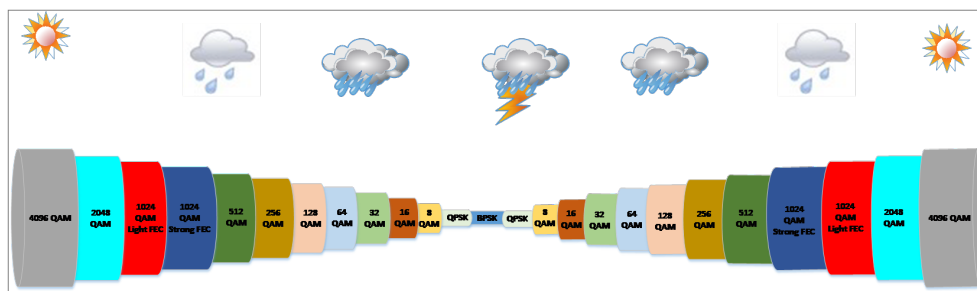
Figure 16: Adaptive Coding and Modulation with 13 Working Points
