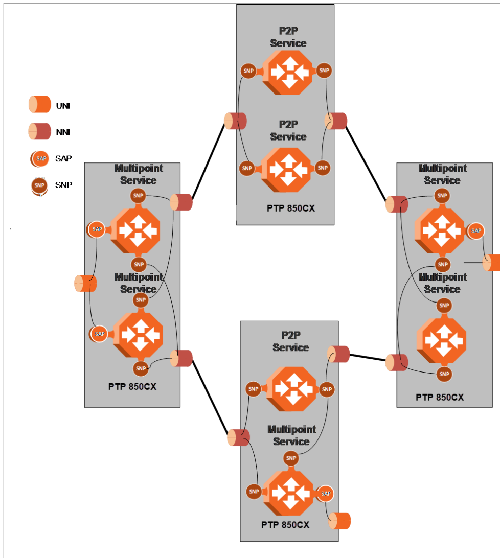
Figure 23: PTP 850CX Services Model
