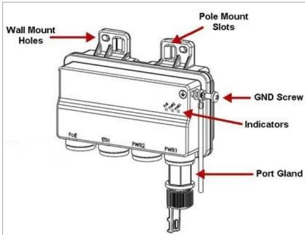
Figure 5: PoE Injector
