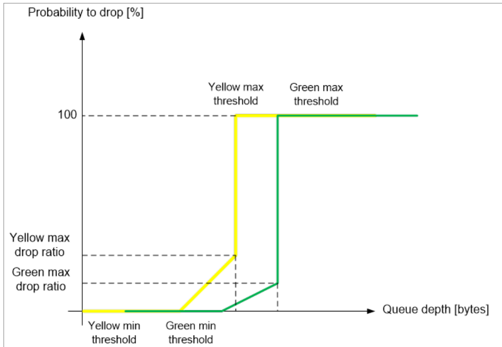
Figure 42: WRED Profile Curve
