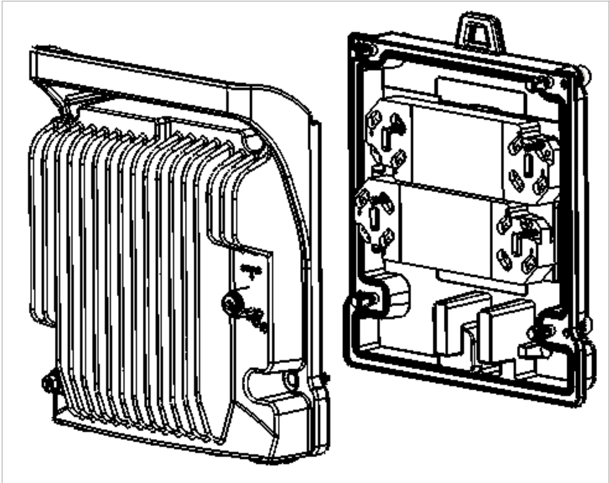
Figure 3: PTP 850CX Radio Unit (Left) and Diplexers Unit (Right)
