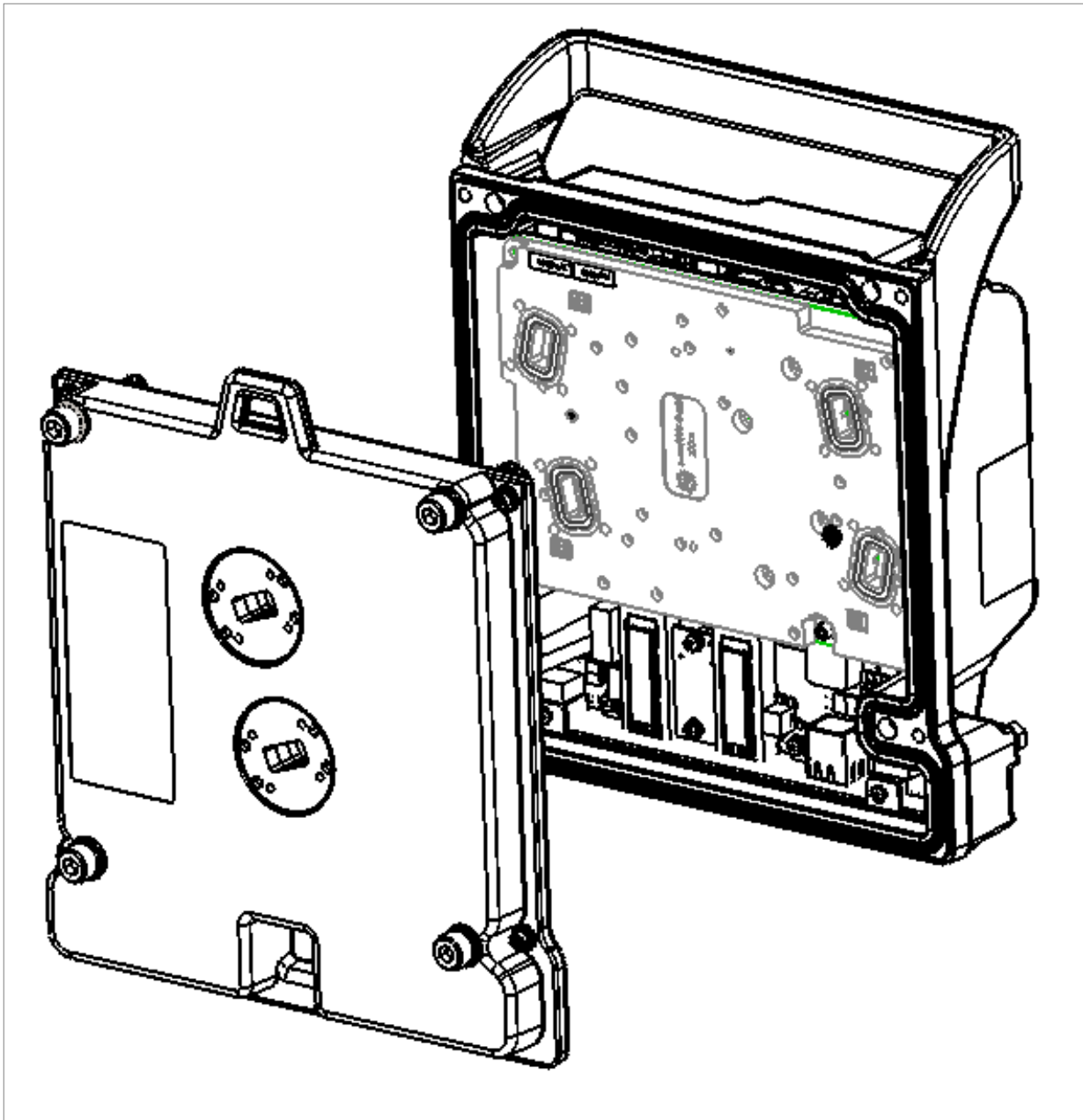
Figure 4: PTP 850CX Radio Unit (Right) and Diplexers Unit (Left)
