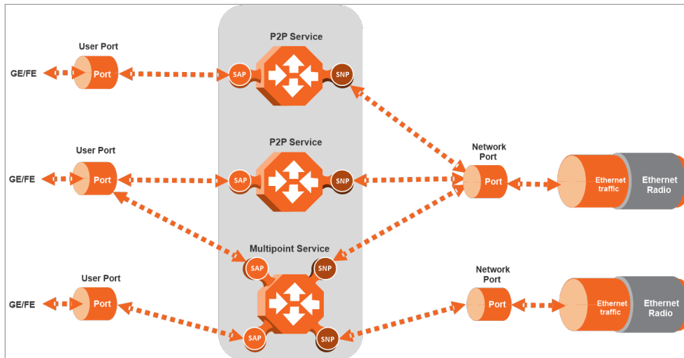
Figure 25: PTP 850CX Services Flow
