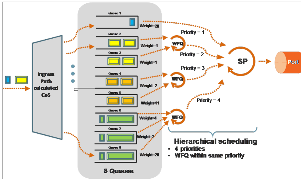
Figure 43: Scheduling Mechanism for a Single Service Bundle
