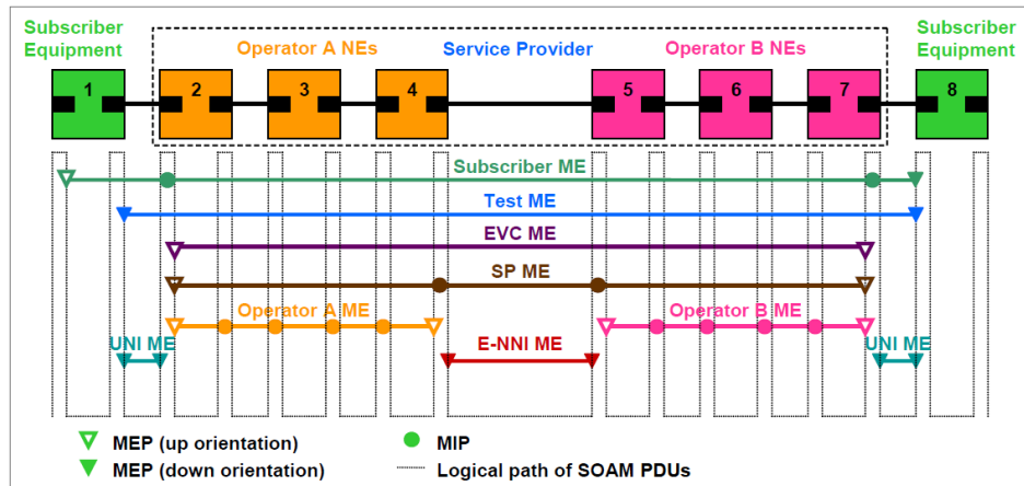
Figure 48: SOAM Maintenance Entities (Example)
