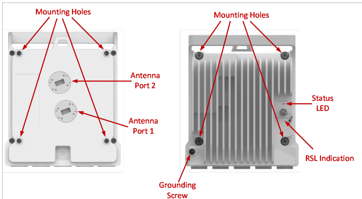
Figure 1: PTP 850CX Rear View (Left) and Front View (Right)
