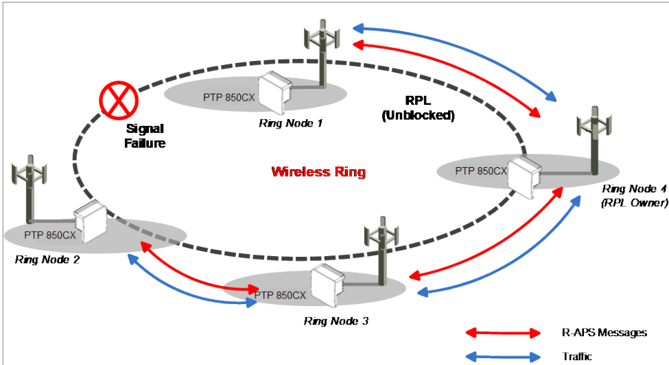
Figure 45: G.8032 Ring in Protecting State
