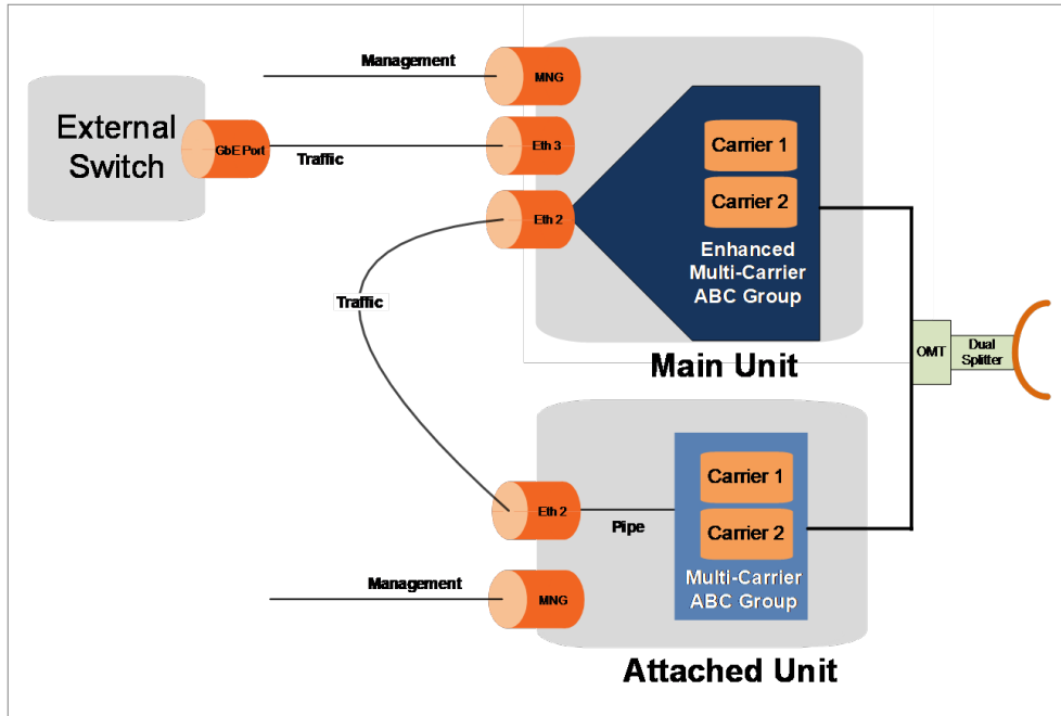
Figure 13: 4+0 Layer 1 Link Aggregation
