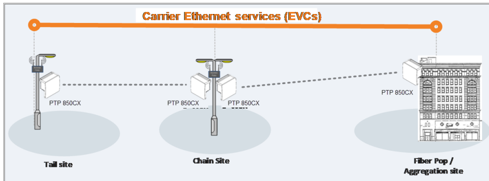
Figure 47: PTP 850CX End-to-End Service Management
