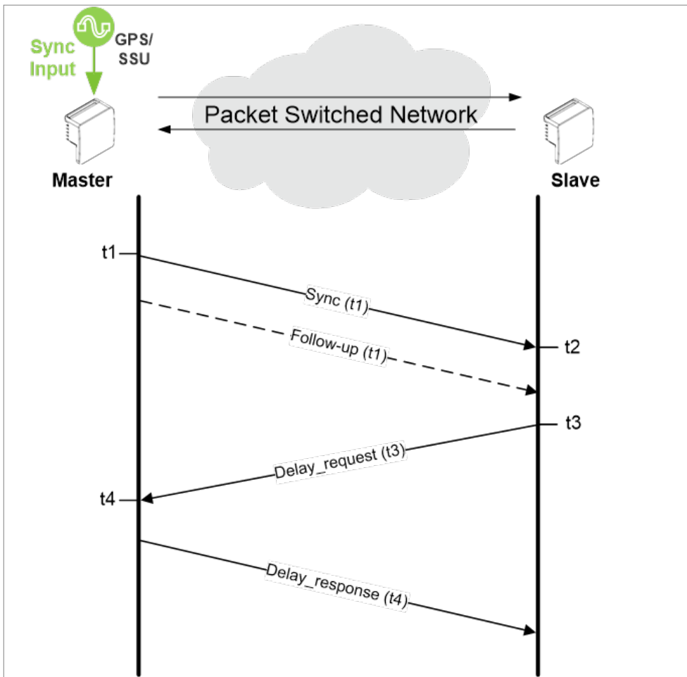
Figure 50: Calculating the Propagation Delay for PTP Packets
