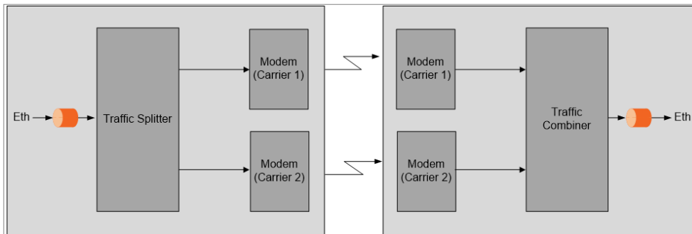
Figure 11: Enhanced Multi-Carrier ABC Traffic Flow
