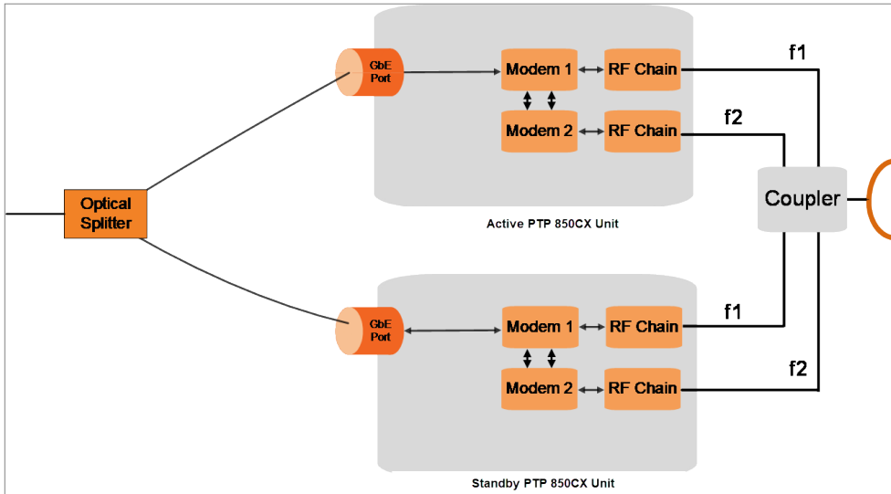
Figure 21: 2+2 Unit Redundancy and HSB – Line Protection Mode
