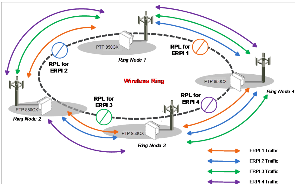
Figure 46: Load Balancing Example in G.8032 Ring
