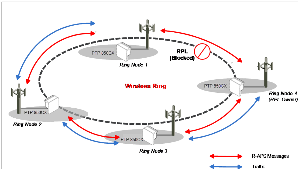
Figure 44: G.8032 Ring in Idle (Normal) State
