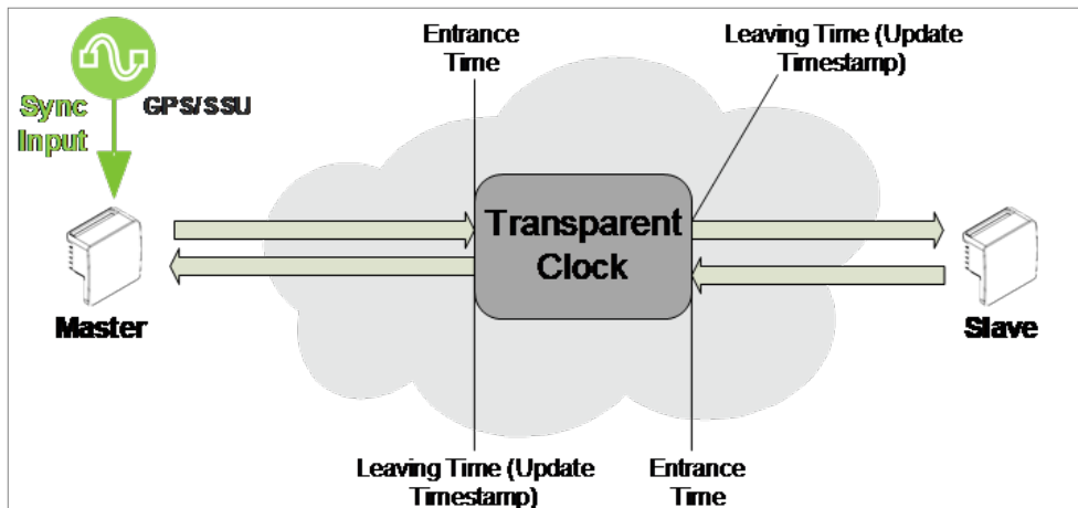
Figure 51: Transparent Clock – General Architecture
