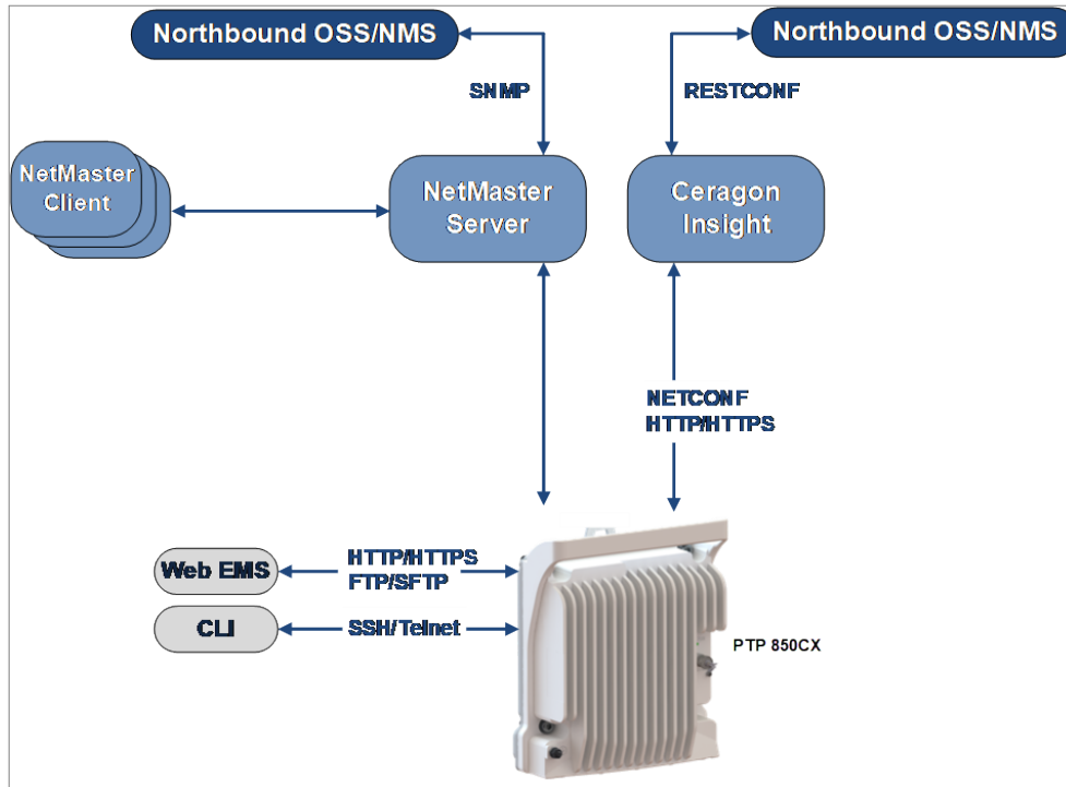
Figure 55: Integrated Management Tools
