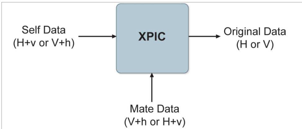
Figure 19: XPIC – Impact of Misalignments and Channel Degradation
