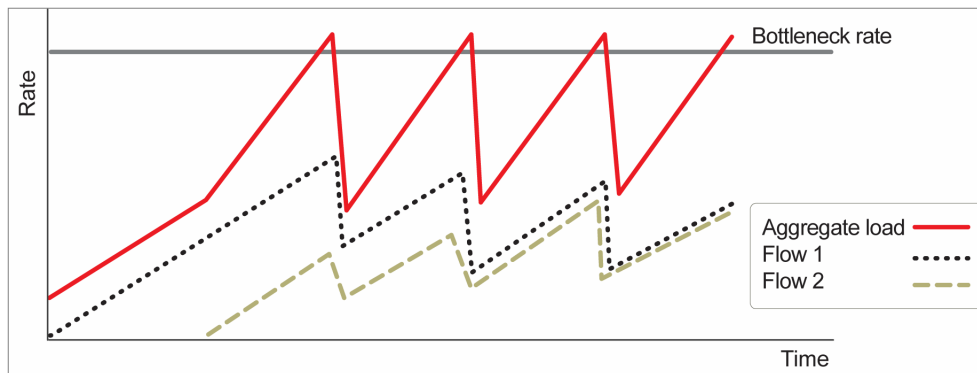
Figure 40: Synchronized Packet Loss
