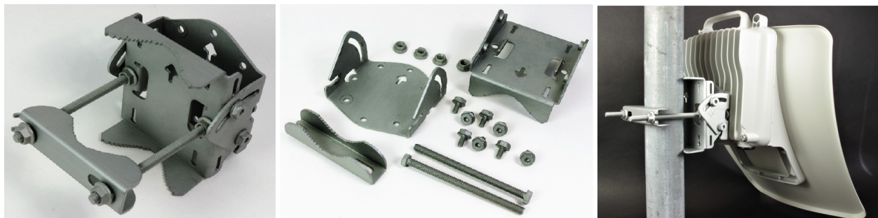
Figure 10 : Tilt bracket assembly
