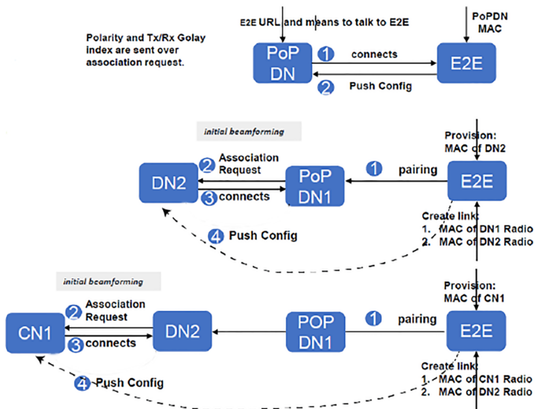
Figure 31: Nodes' deployment
