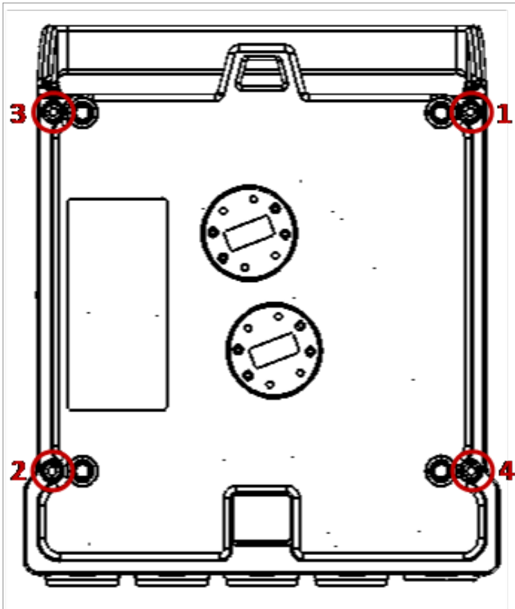
Figure 23: Tightening the Screws From the Diplexer Side Unit
