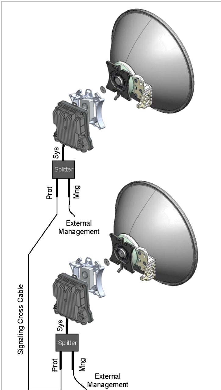
Figure 19: 2x2 HSB Protection Configuration with External Management
