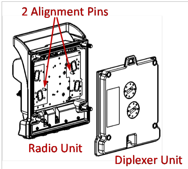
Figure 22: Attaching the Diplexer
