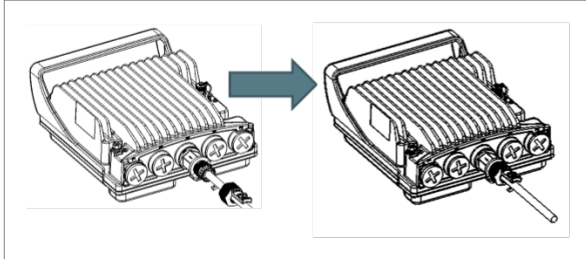
Figure 17: Tightening the Front Portion of the Gland and Tightening the Rear Portion of the Gland
