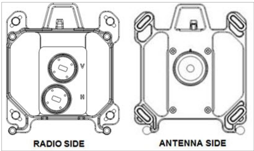
Figure 4: OMT
