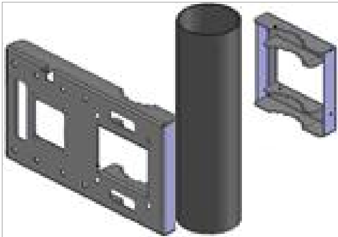
Figure 11: Remote Dual Pole Mount
