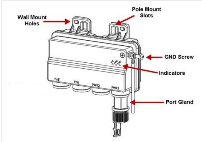
Figure 5: PoE Injector
