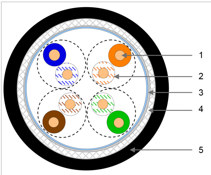
Figure 16: Cable Design
