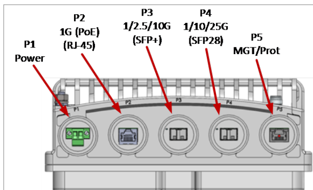
Figure 2: PTP 850CX Interfaces
