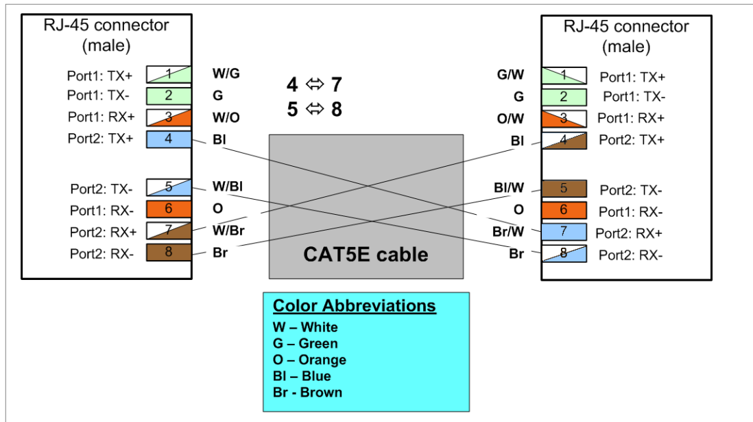
Figure 18: Protection Signaling Cable Pinouts
