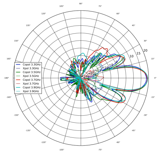
3 GHz Elevation
