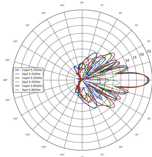
5 GHz Azimuth
