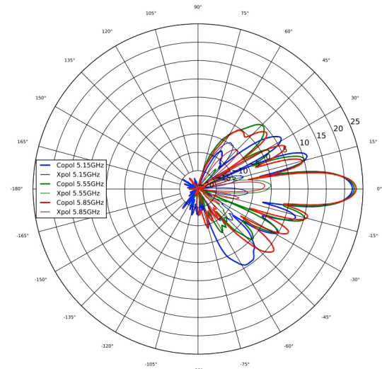
5 GHz Elevation
