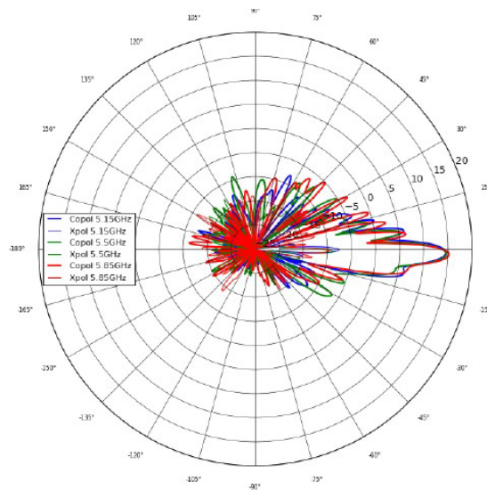
CH 6 Horizontal Polarization, Elevation
