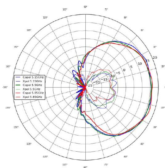
CH 5 Vertical Polarization, Azimuth
