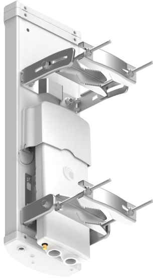
Figure 6: ePMP 4600 Access Point module mounting bracket
