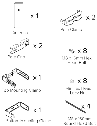
Figure 8: 4x4 Sector Antenna
