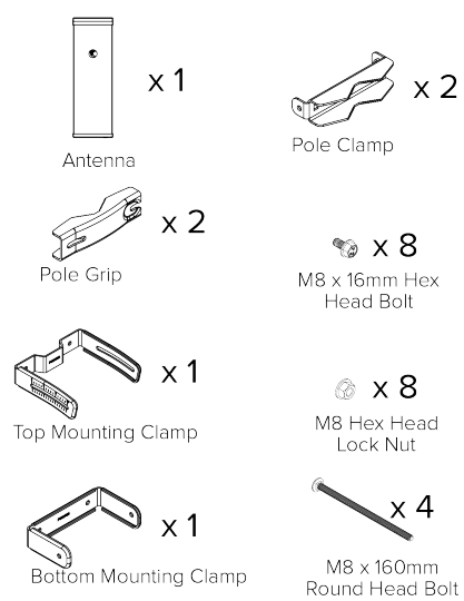
Figure 8: 4x4 Sector Antenna (Optional)
