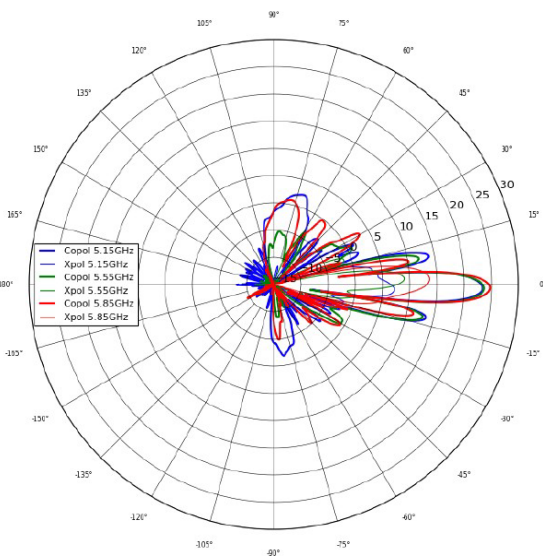
Elevation Horizontal
